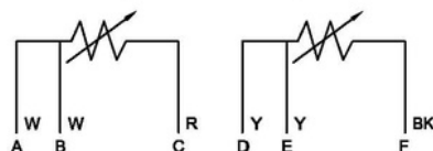
DUAL 6-WIRE WIRING DIAGRAM
