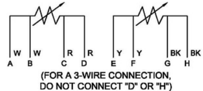
DUAL 4-WIRE WIRING DIAGRAM
